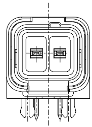
Keying No.Y
